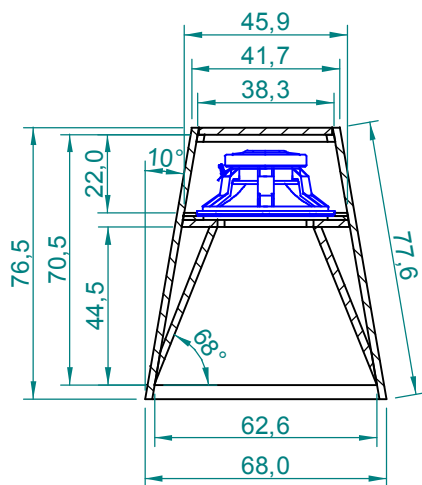
Section C-C
